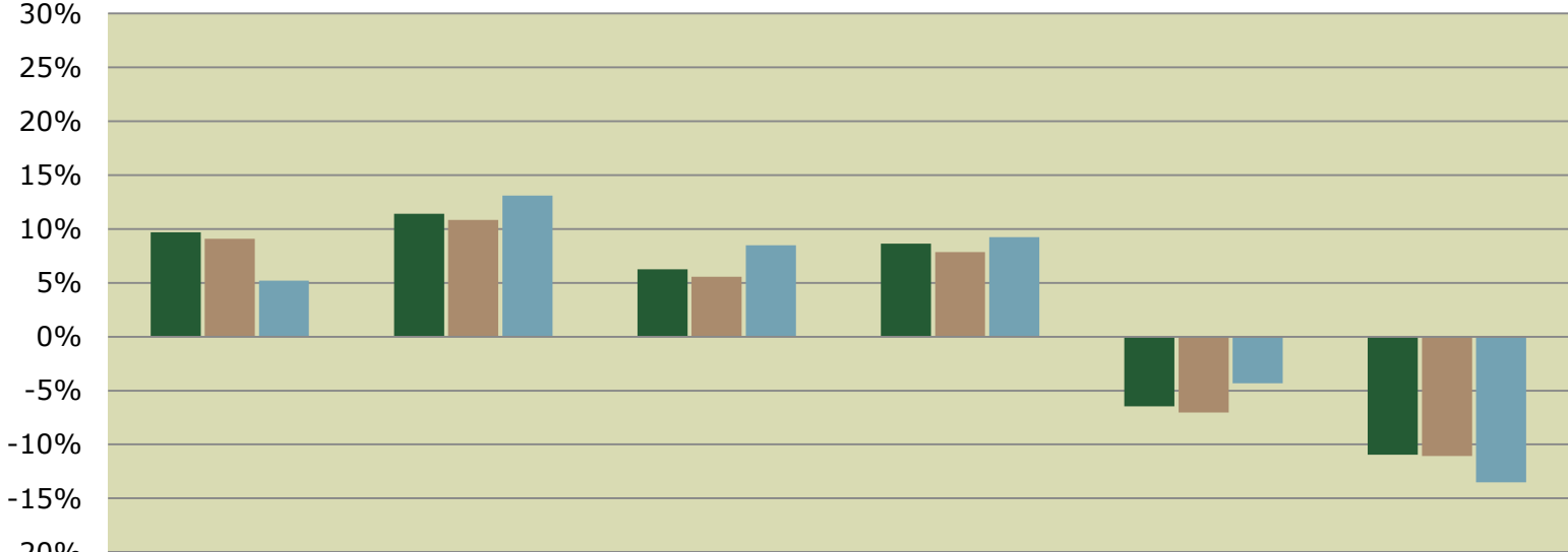
Annual Performance
